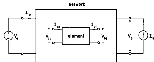
Fig. 1. Sign convention used.
